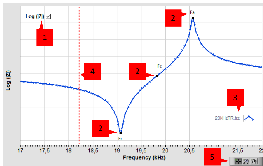
Log(|Z|) graph as a function of frequency with the main elements numbered.
