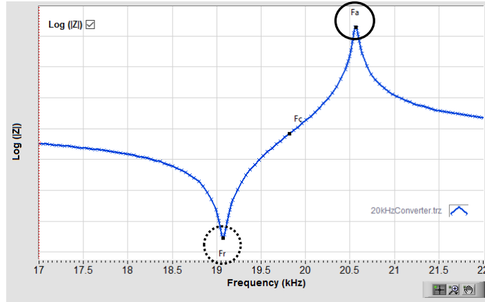
Typical curve of the impedance modulus as a function of frequency ( |Z(f)| ). The resonance frequency is highlighted by a dotted circle, and the antiresonance frequency by a continuous circle.
