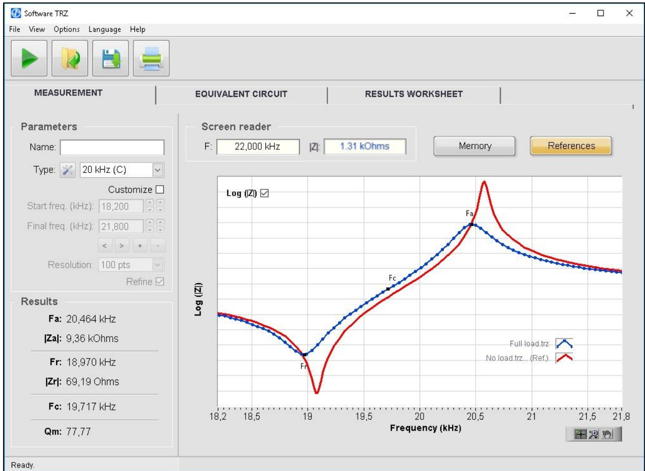
Example of use of the "Reference" function (reference curve is shown in red).
