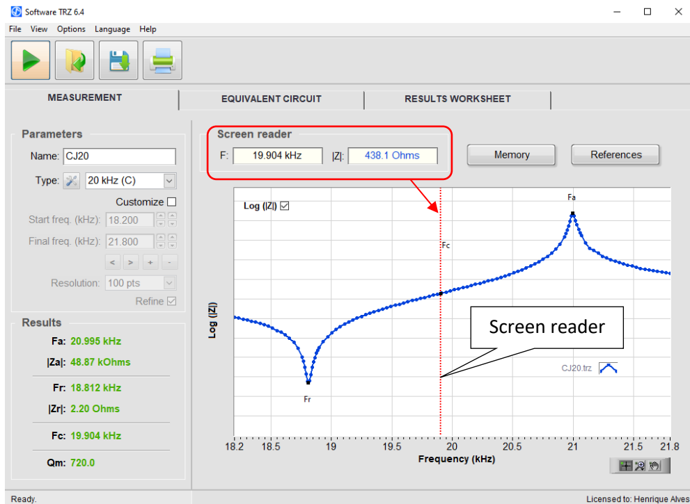
Frequency and impedance modulus ( |Z| ) at the position of the screen reader.
